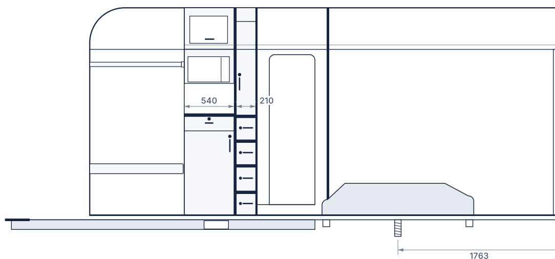
INTERIOR SIDE VIEW
