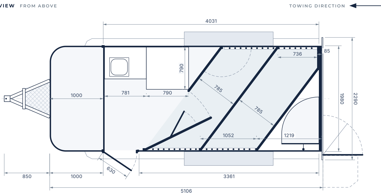
PLAN VIEW FROM ABOVE
