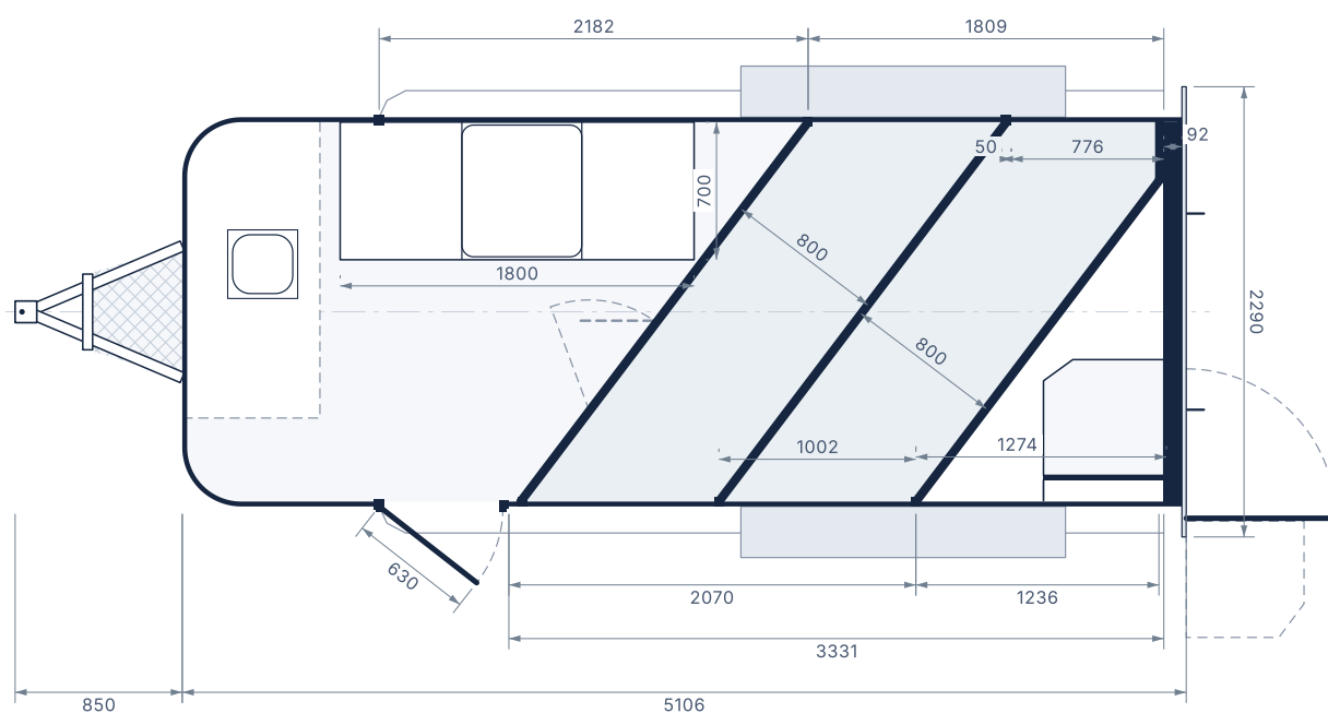
PLAN VIEW FROM ABOVE
